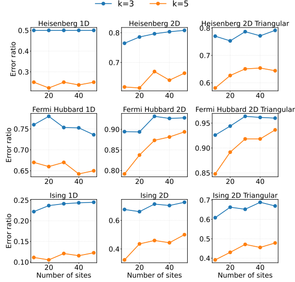
Fig. 10: Ratio quantifying percentage reduction of non-commuting pairs of Hamiltonian terms between partitioned and unpartitioned Hamiltonians over increasing quantum lattice sizes.
