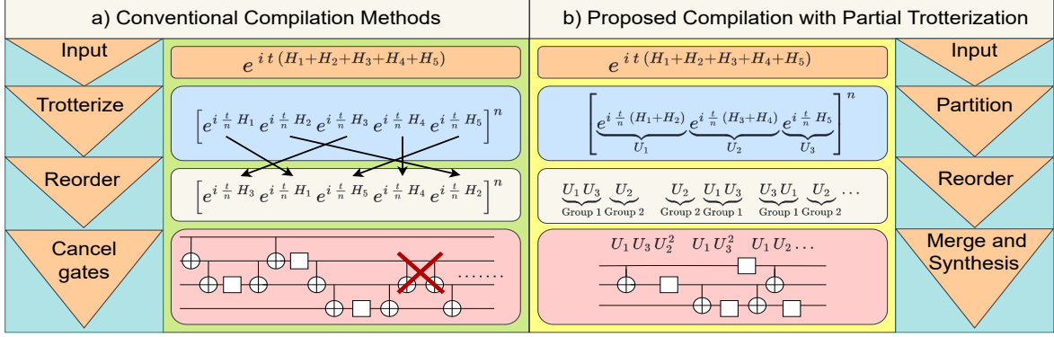
Fig. 1: a) Conventional compilation flow vs b) the proposed Kernpiler compiler. a) The time unitary is split into small unitaries with analytical circuit representations. These unitaries are reordered to take advantage in circuit representation structure and reduce gates. Finally, the reordered Trotter step is lowered into the gate representation with no change in error bound. b) Pipeline for reducing gates through error term reduction. First we group into partial Trotter steps which act on a subset of N qubits, in our case N=3 . Then we perform an efficient numerical rewrite of the partial Trotter unitaries. Next step, group into commuting subsets of unitaries placing the largest two groups of unitaries on the edges of the Trotter step. Finally, we use a partially symmetric Trotter step to cancel error terms in the expansion by alternating every other Trotter steps order. Commuting unitaries then merge back together naturally allowing for a unitary reduction with no additional error. The compilation finishes at circuit-level.
