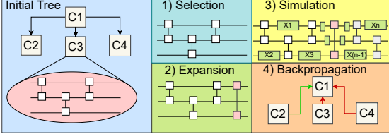
Fig. 4: Unitary decomposition method 1) Selection : Select a node in the search tree which represents a partially synthesized circuit which has unexplored child actions. 2) Expansion : Select a CNOT gate among choices from the gateset to append to the circuit. 3) Simulation : Starting from the newly expanded state, append CNOTs until we reach a terminal circuit length. After, interleave a fixed number of single qubit gates at random in between the CNOT gates. Optimize parameters with the Gauss-Newton method. 4) Backpropagation : Update values of nodes in the tree based on the result of the simulation stage to identify if the newly explored state was valuable.
