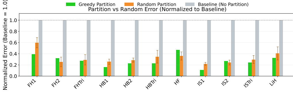
Fig. 8: Normalized comparison of error saved when comparing different partitioning strategies. These strategies include random, greedy, and no partitioning
