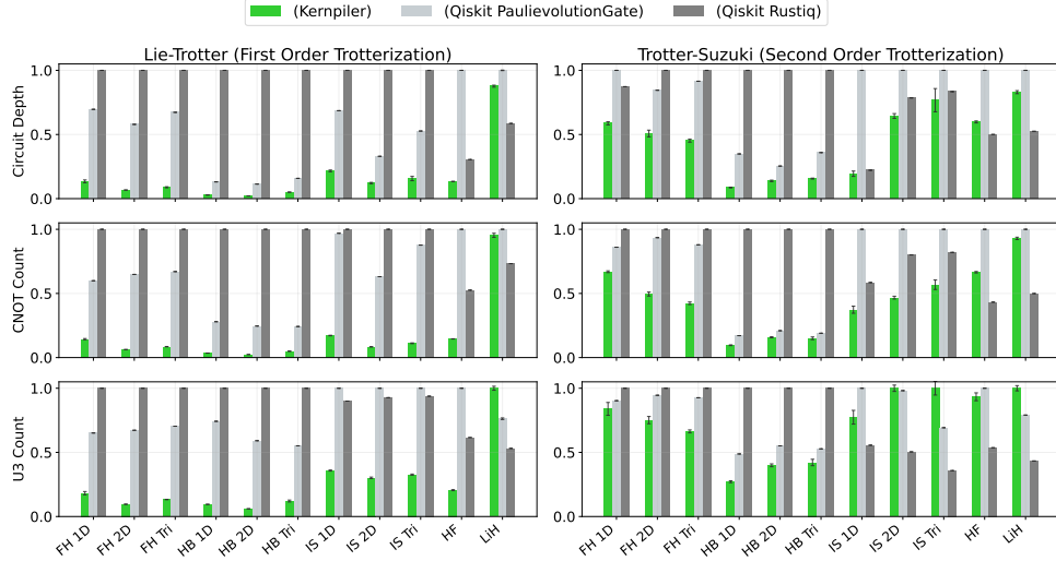
Fig. 6: Depth, CNOT and U3 count comparison when compiling to less than 1% approximation error on a range of time evolution unitaries.
