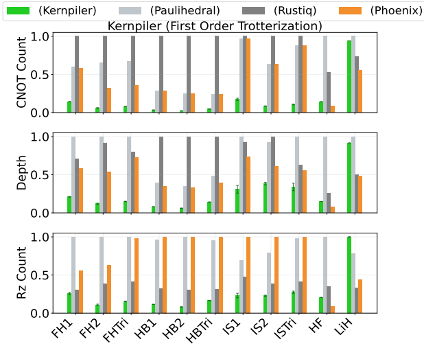
Fig. 7: Circuit Depth, CNOT and Rz count comparison when compiling to less than 1% approximation error on a range of time evolution unitaries.
